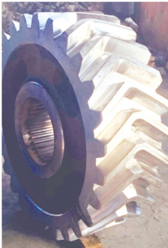
电铲人字齿/ Double Helical Tooth M=36 \Phi=1.4m
