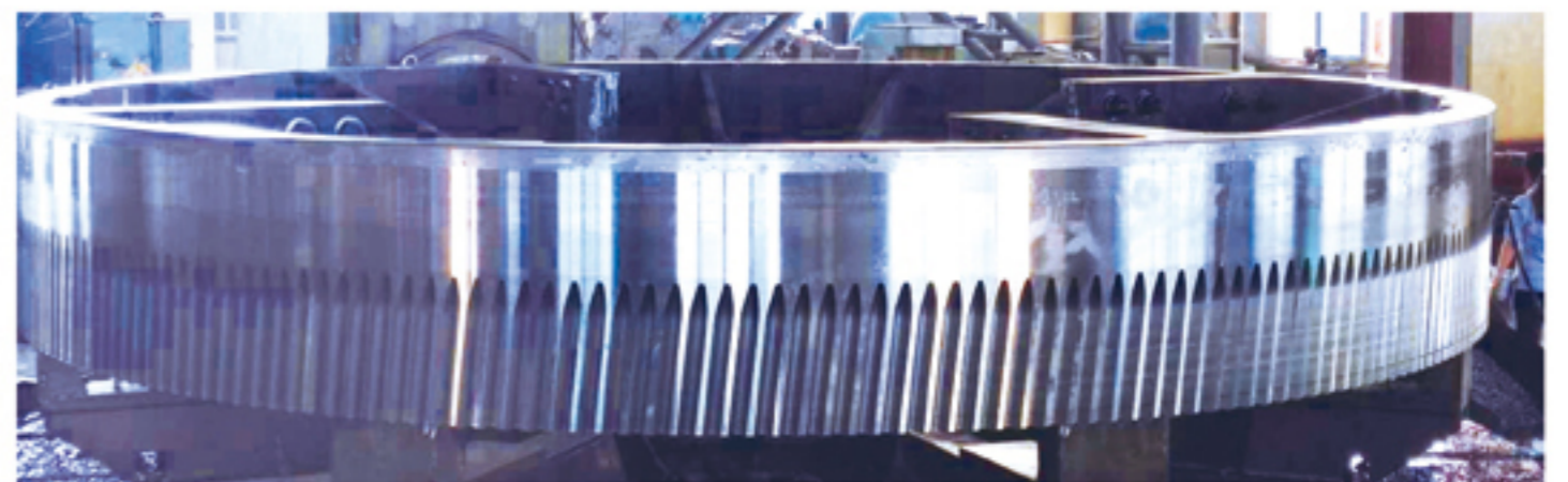
齿圈/ Girth Gear M=20 \Phi=6.4m
